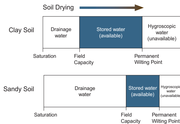
FIGURE 2.18. Water storage for two soil textural groups. The blue shaded area represents water that is available for plant use.
