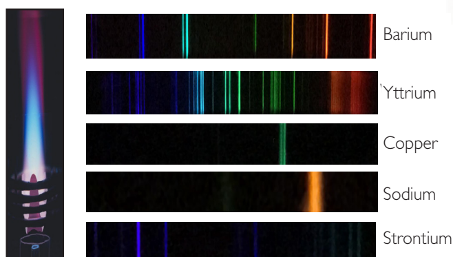
(Left) Heavy metal samples are analyzed by an inductively coupled plasma (ICP) instrument. (Right) Every element has a unique spectrum that can be identified and quantified.
