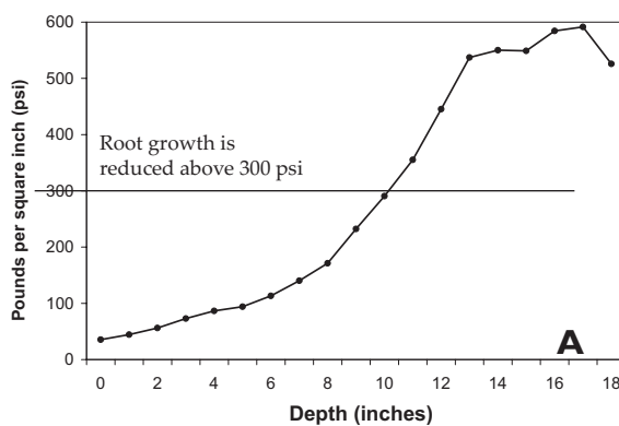
FIGURE 2.21 A and B. Soil compaction graphs for (A) a field in intensive vegetable production and (B) a conventionally plow-tilled field and zone-till field with deep ripping on the same farm in the spring of 2005 (Courtesy of C.R. MacNeil).
