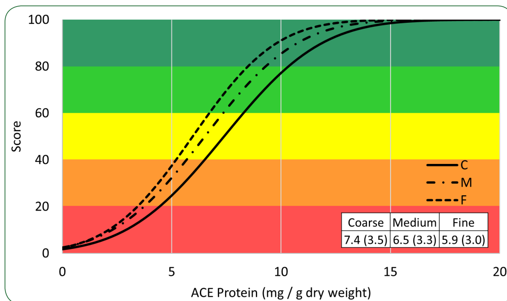
FIGURE 2.34. ACE Soil Protein Index scoring functions and upper value limits for Coarse (C), Medium (M) and Fine (F) textural classes. Mean and standard deviation (in parenthesis) for each class are provided. In this case more is better. Higher protein index scores indicate a larger pool of organically-bound N in the soil.
