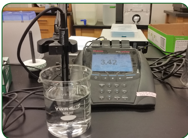
FIGURE 2.52. Electrical conductivity (EC) meter used to measure salinity.
