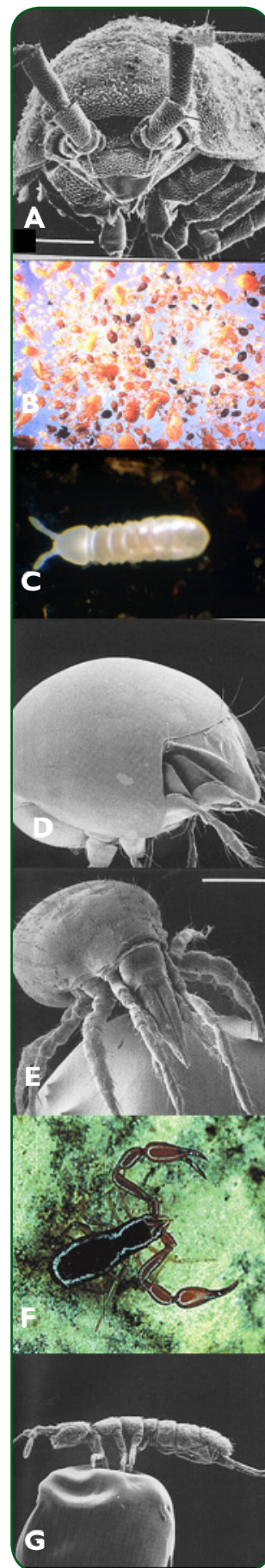
FIGURE I.07. Various Arthropods feed on decaying OM and break larger pieces down into smaller ones: A) Sowbug, B) 200 species of mites, C & G) springtail, D) Oribatid turtle-mite, E) Predatory Pergamasus mite, F) Pseudoscorpion. Photos credit: Soil and Water Conservation Society
