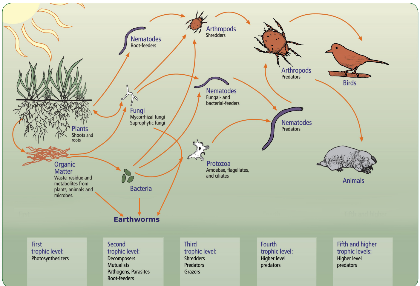
FIGURE I.06. The soil food web. Relationship between the soil food web, plants, organic matter and animals. Adapted from USDA- NRCS
