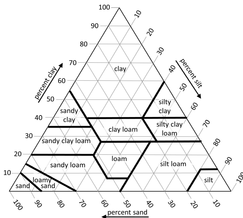
FIGURE 1.04. The soil textural triangle. For example, a soil with a texture of 70% silt, 20% sand, and 10% clay can be classified as a silt loam, one of the textural classes. Adapted from USDA-NRCS
