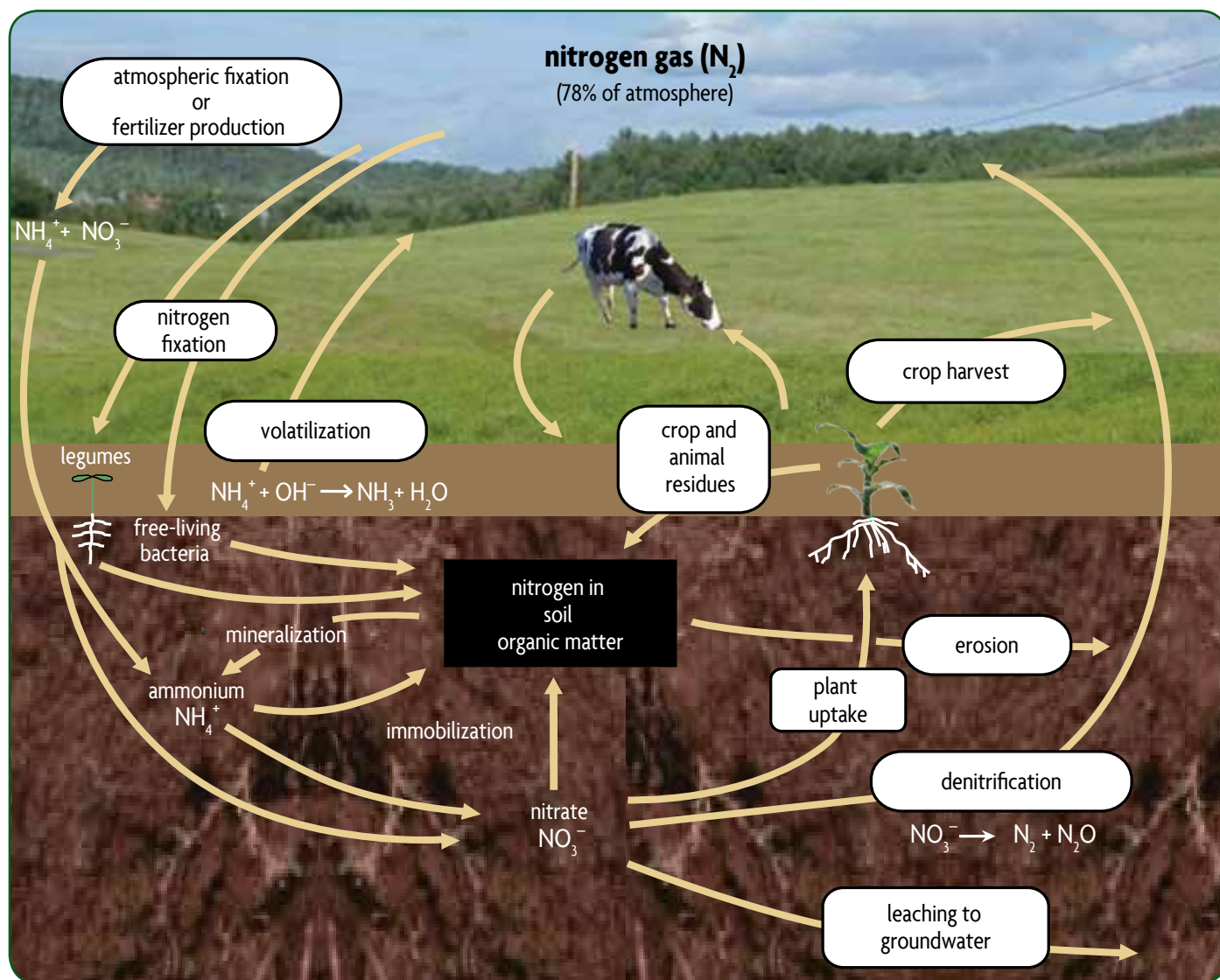
FIGURE 1.10. Nitrogen cycle demonstrating nutrient benefits from decomposition.
