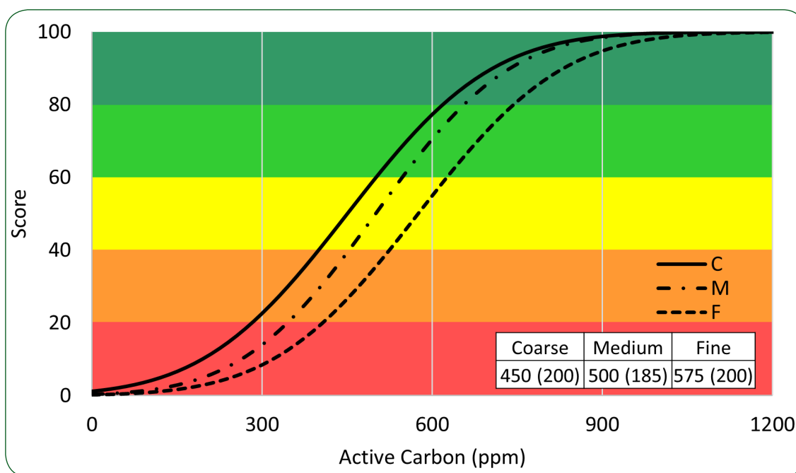
FIGURE 2.38. Active carbon scoring functions and upper value limits for Coarse (C), Medium (M) and Fine (F) textural classes. Mean and standard deviation (in parenthesis) for each class are provided. In this case more is better. Higher active carbon scores indicate a trend toward more organic matter building up in the soil through biological activity.
